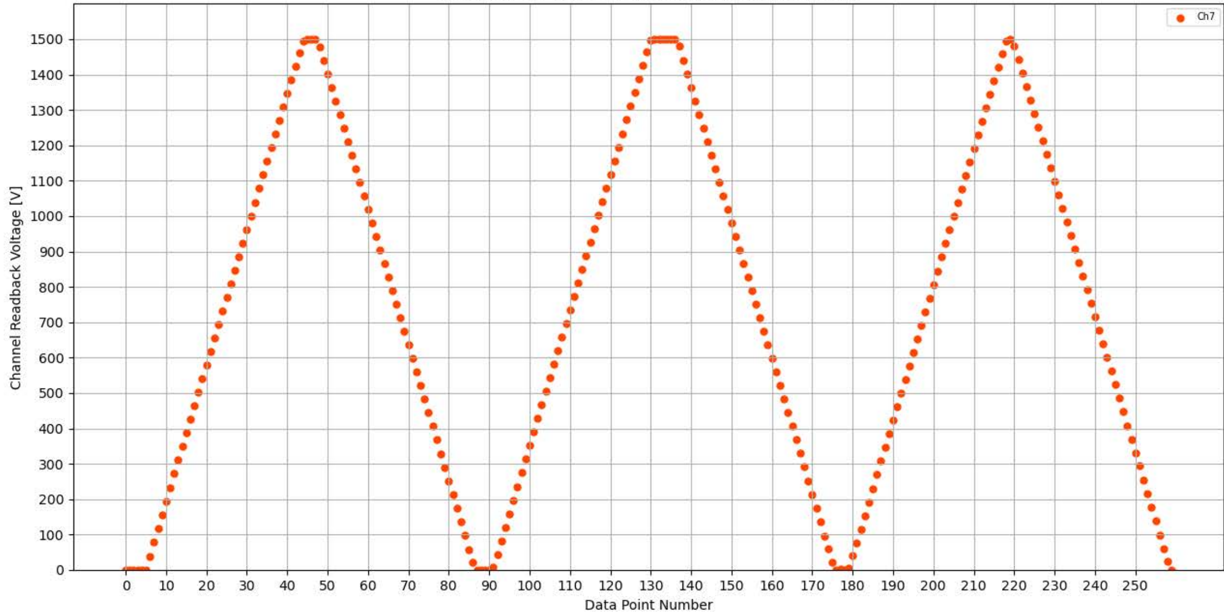
Voltage Ramp Test (Python) Bd #355, Slot #5, Ch #7
