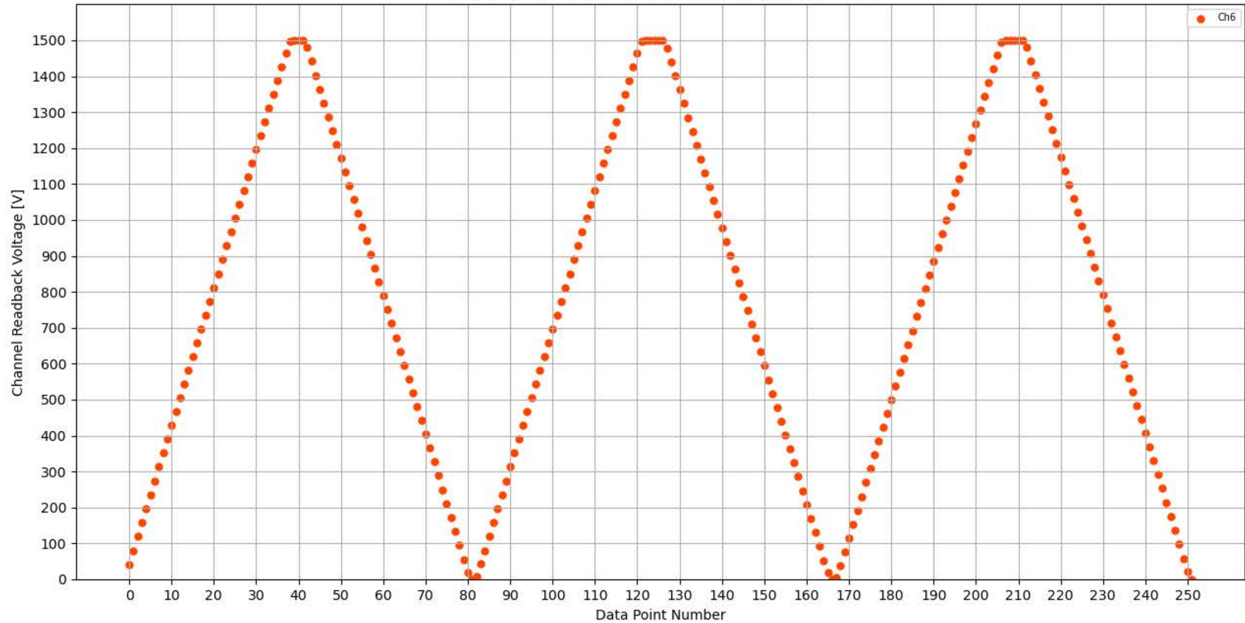
Voltage Ramp Test (Python) Bd #355, Slot #5, Ch #6
