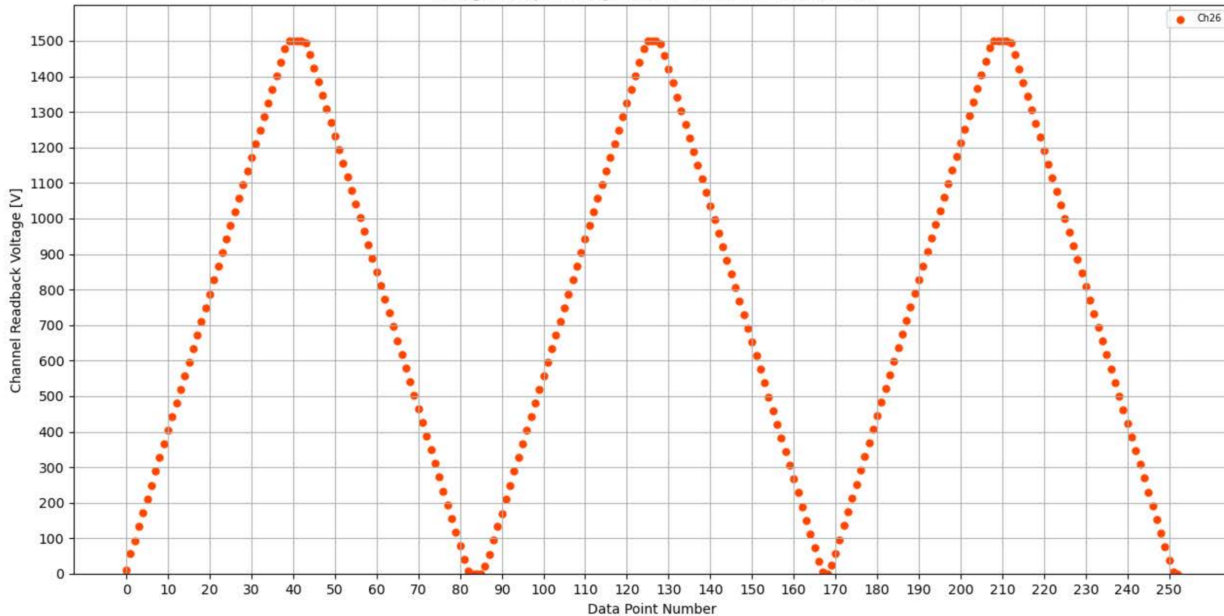
Voltage Ramp Test (Python) Bd #355, Slot #5, Ch #26
