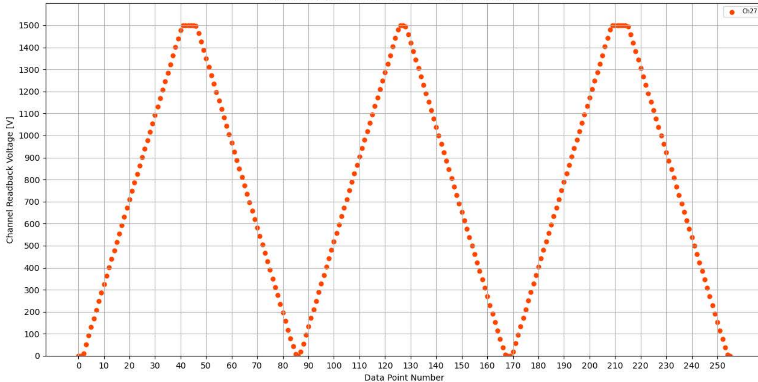
Voltage Ramp Test (Python) Bd #355, Slot #5, Ch #27
