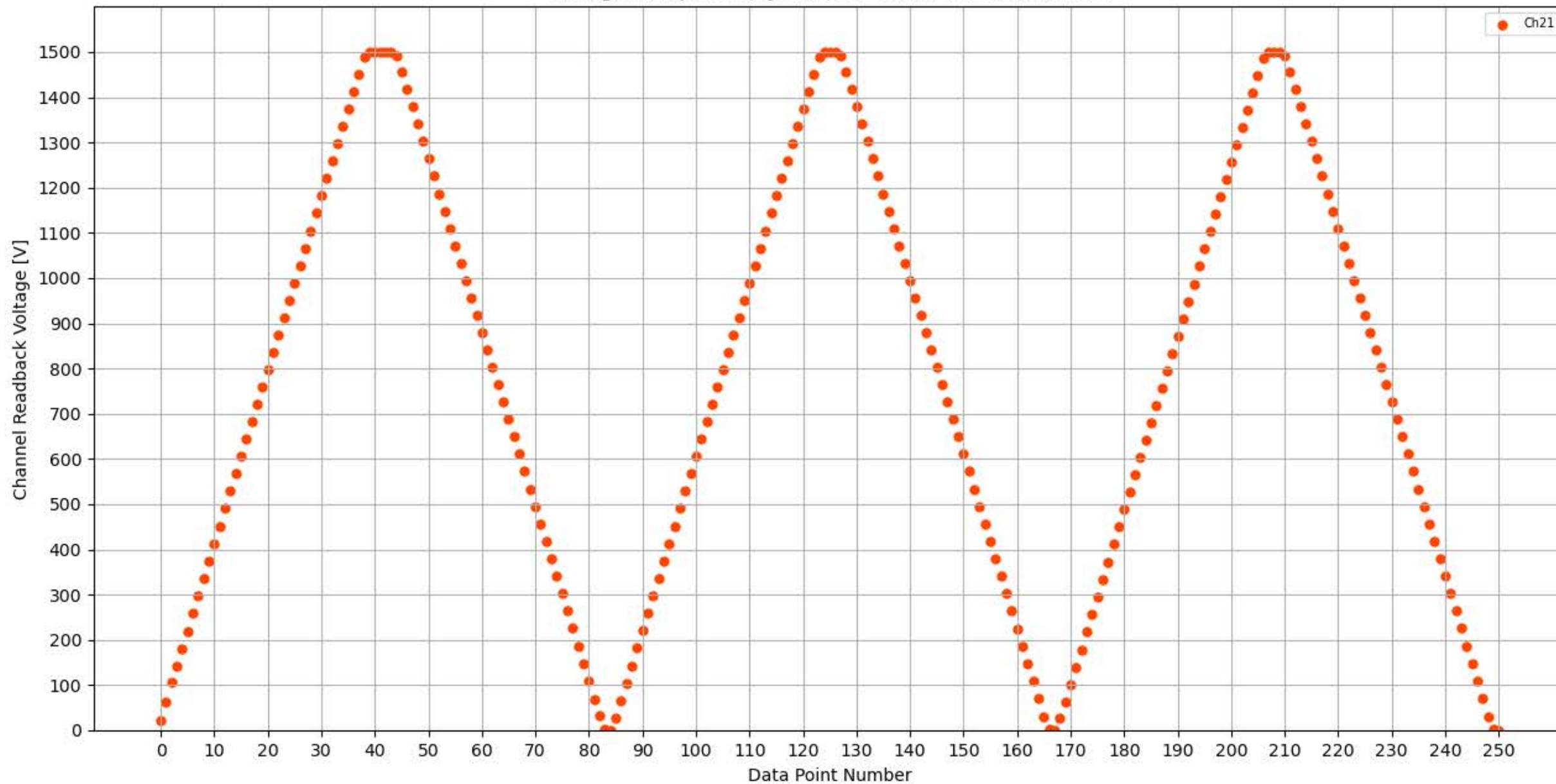
Voltage Ramp Test (Python) Bd #355, Slot #5, Ch #21
