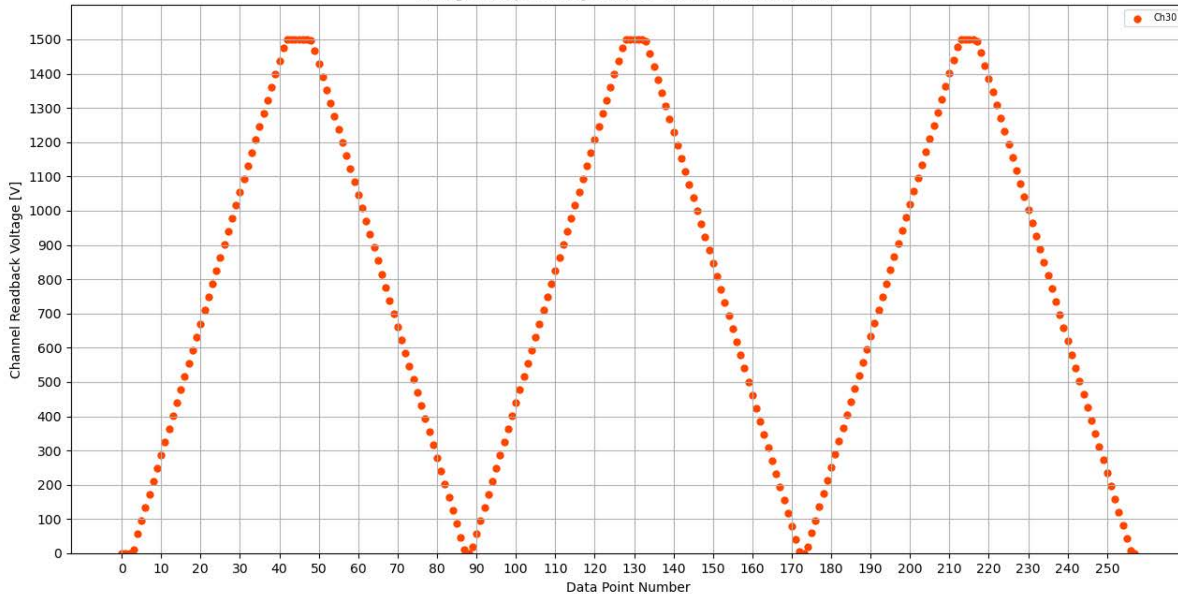
Voltage Ramp Test (Python) Bd #355, Slot #5, Ch #30
