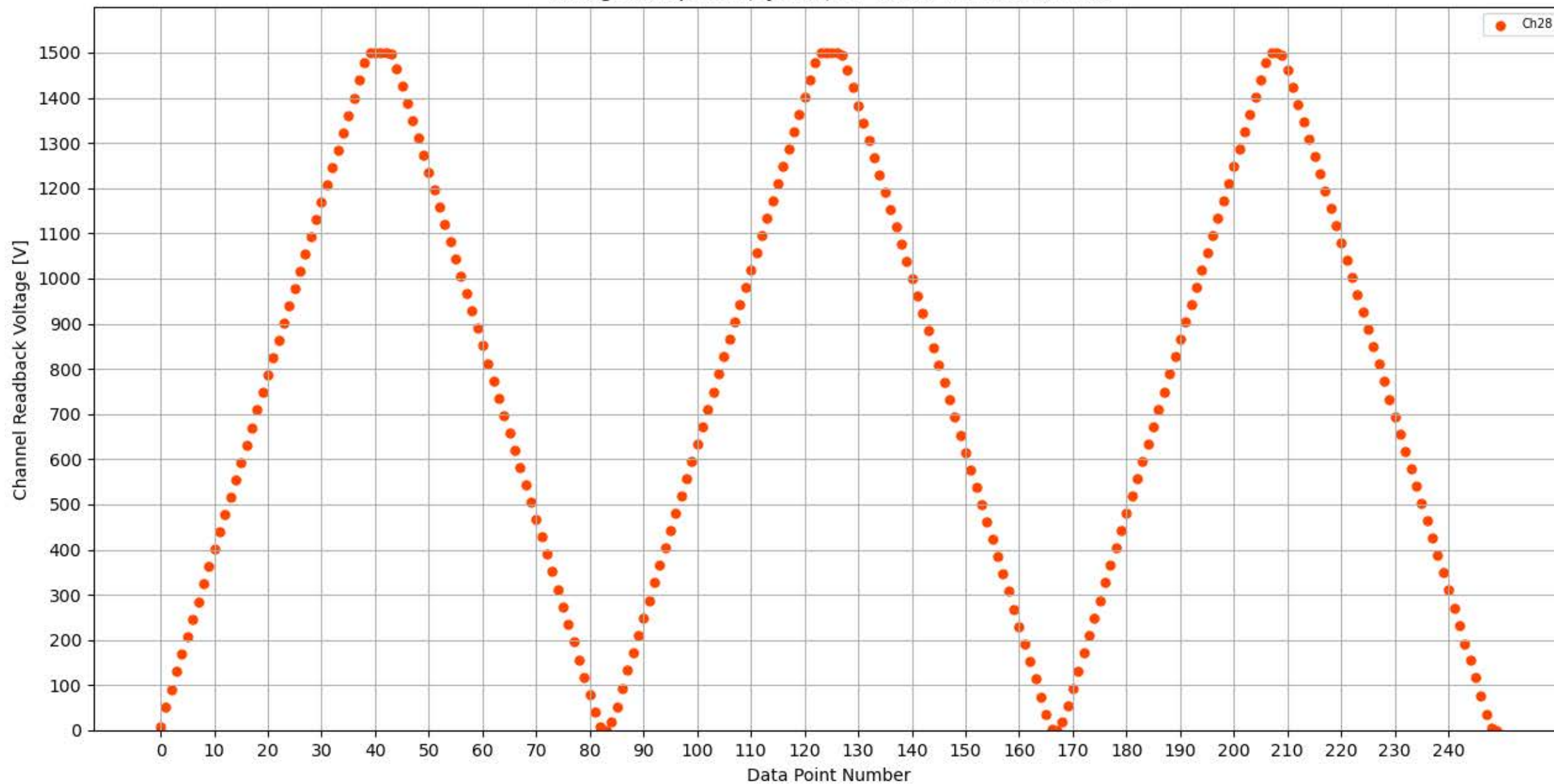
Voltage Ramp Test (Python) Bd #355, Slot #5, Ch #28
