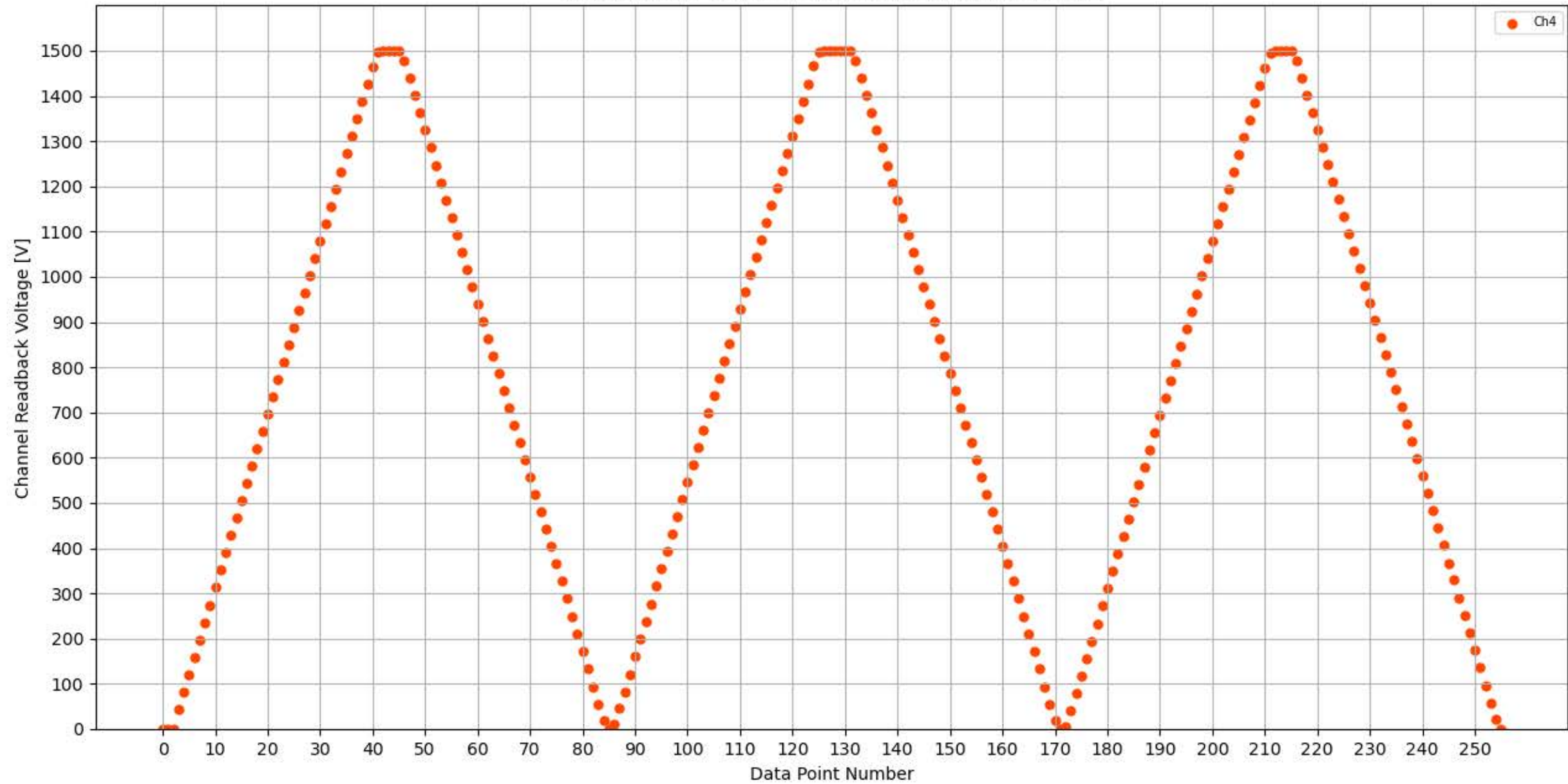
Voltage Ramp Test (Python) Bd #355, Slot #5, Ch #4
