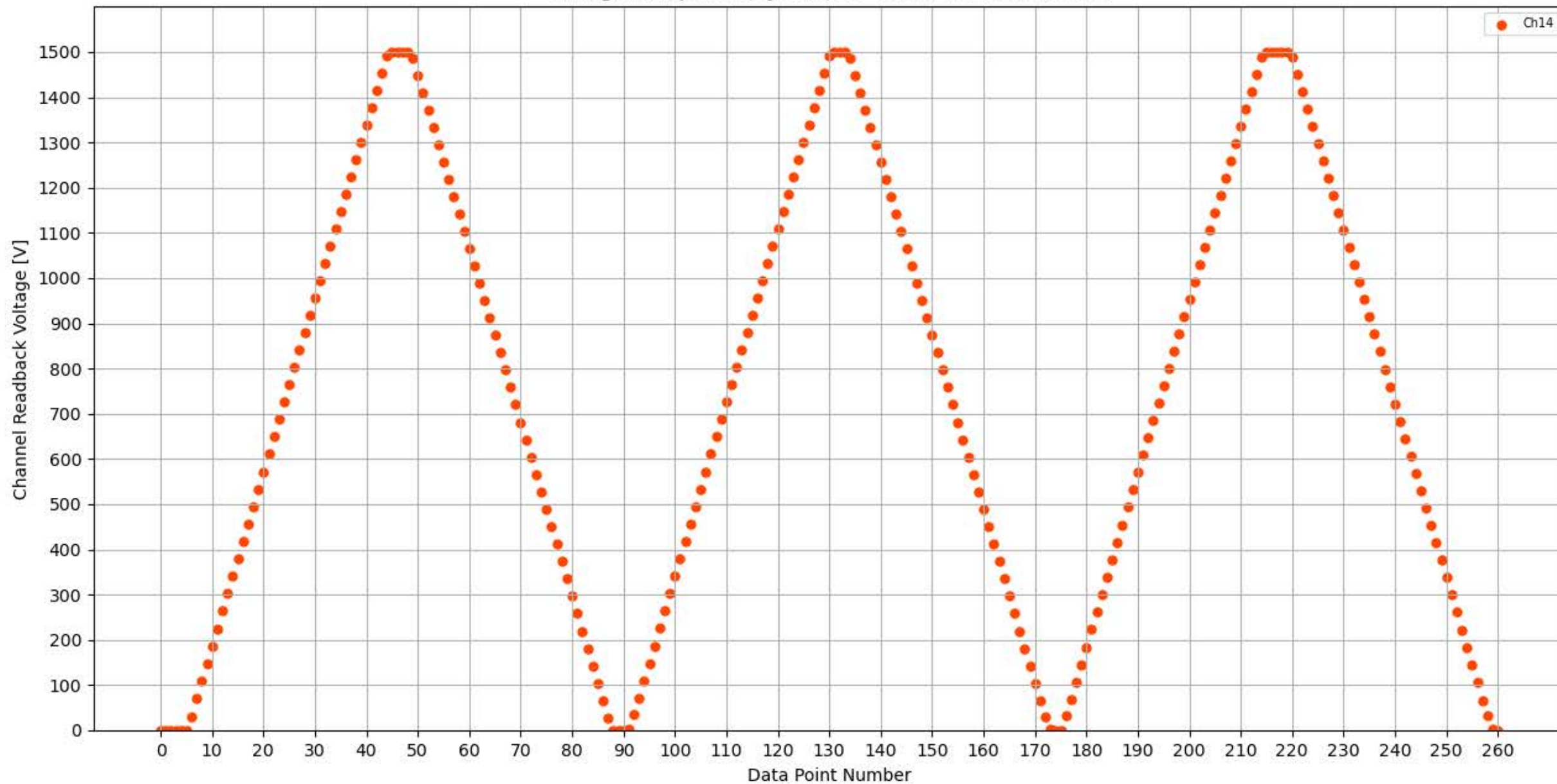
Voltage Ramp Test (Python) Bd #355, Slot #5, Ch #14
