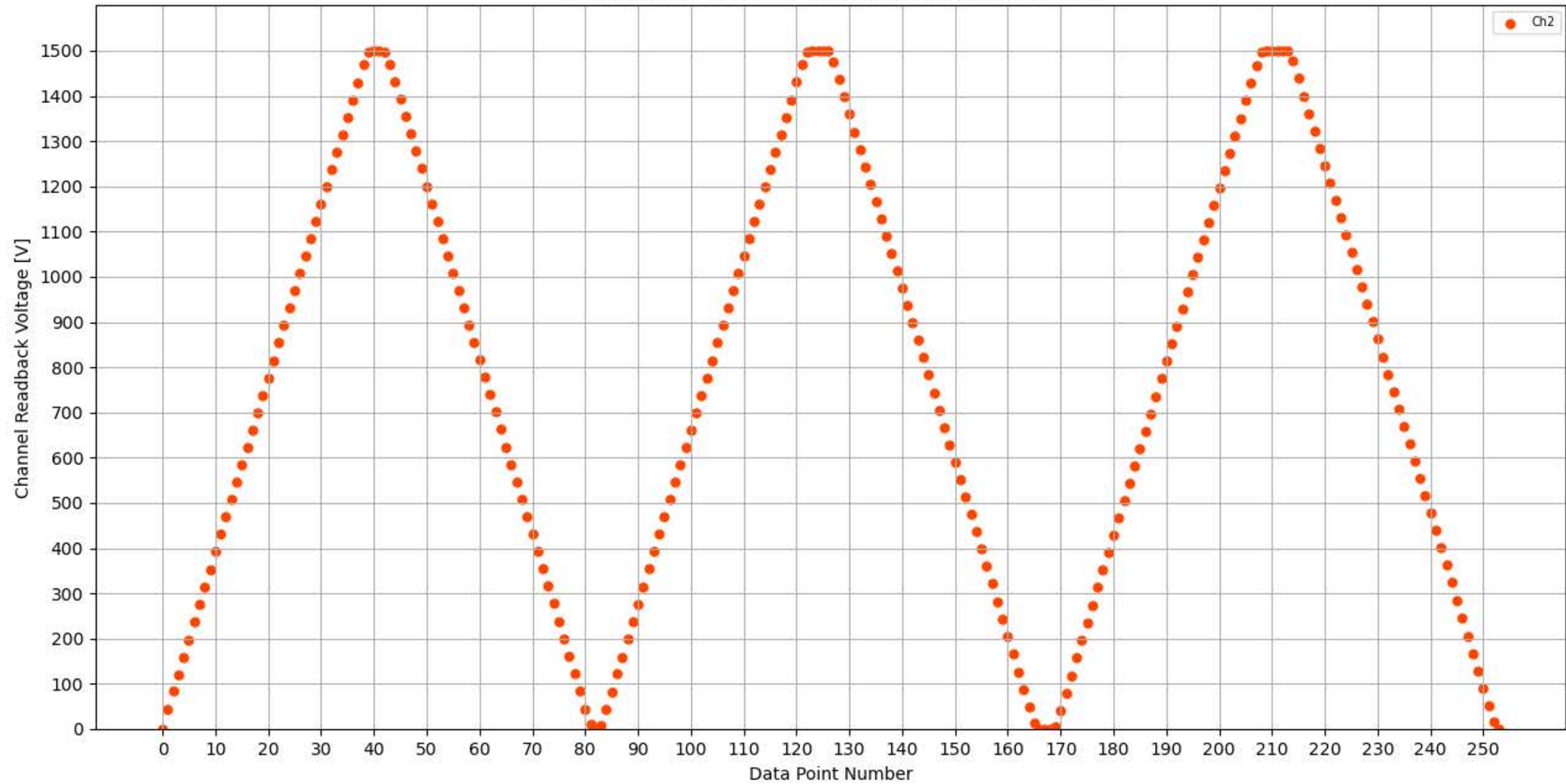
Voltage Ramp Test (Python) Bd #355, Slot #5, Ch #2
