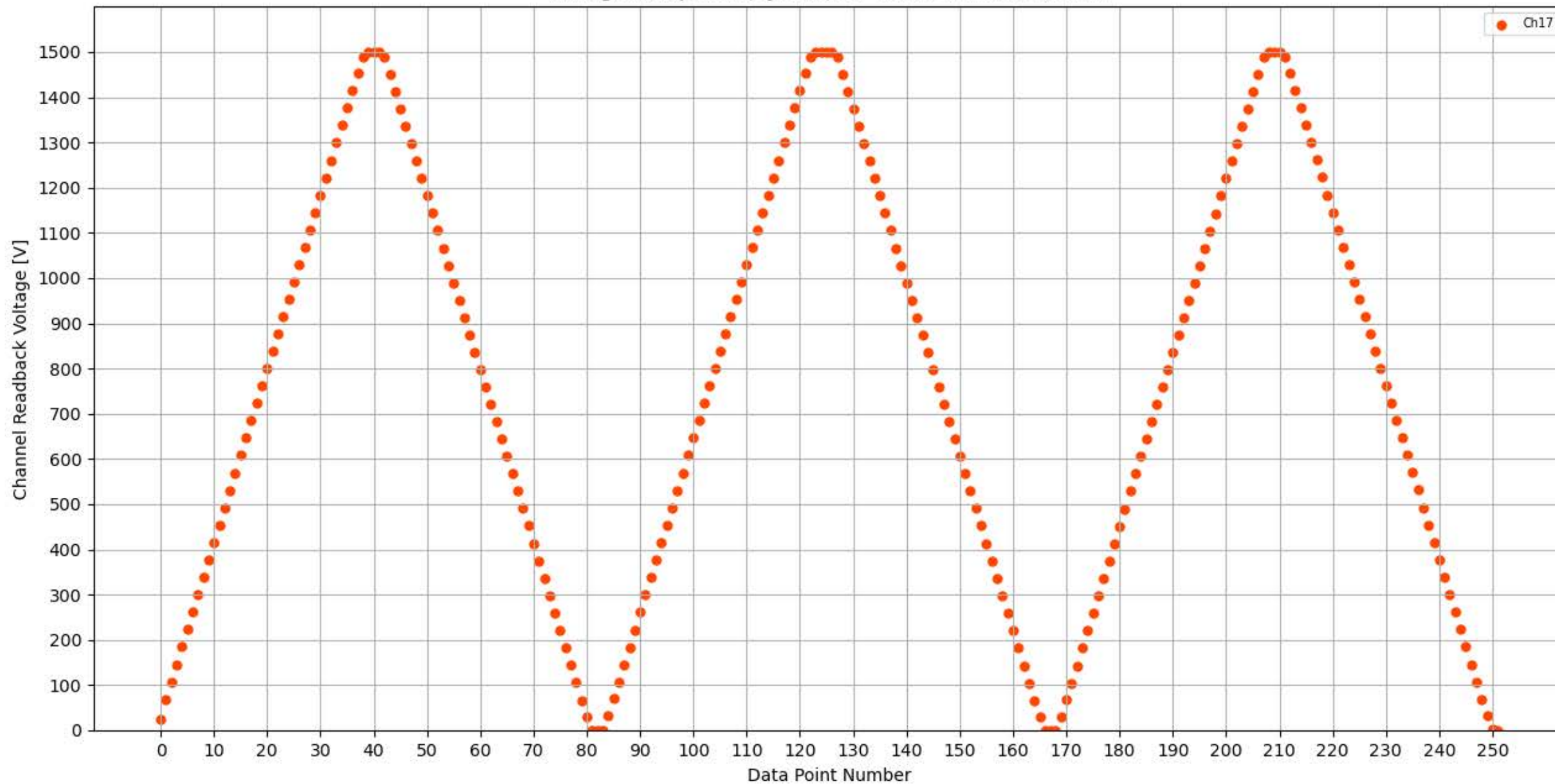
Voltage Ramp Test (Python) Bd #355, Slot #5, Ch #17
