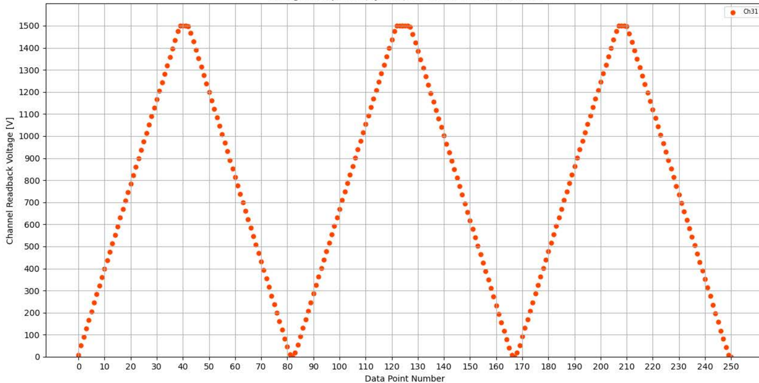
Voltage Ramp Test (Python) Bd #355, Slot #5, Ch #31
