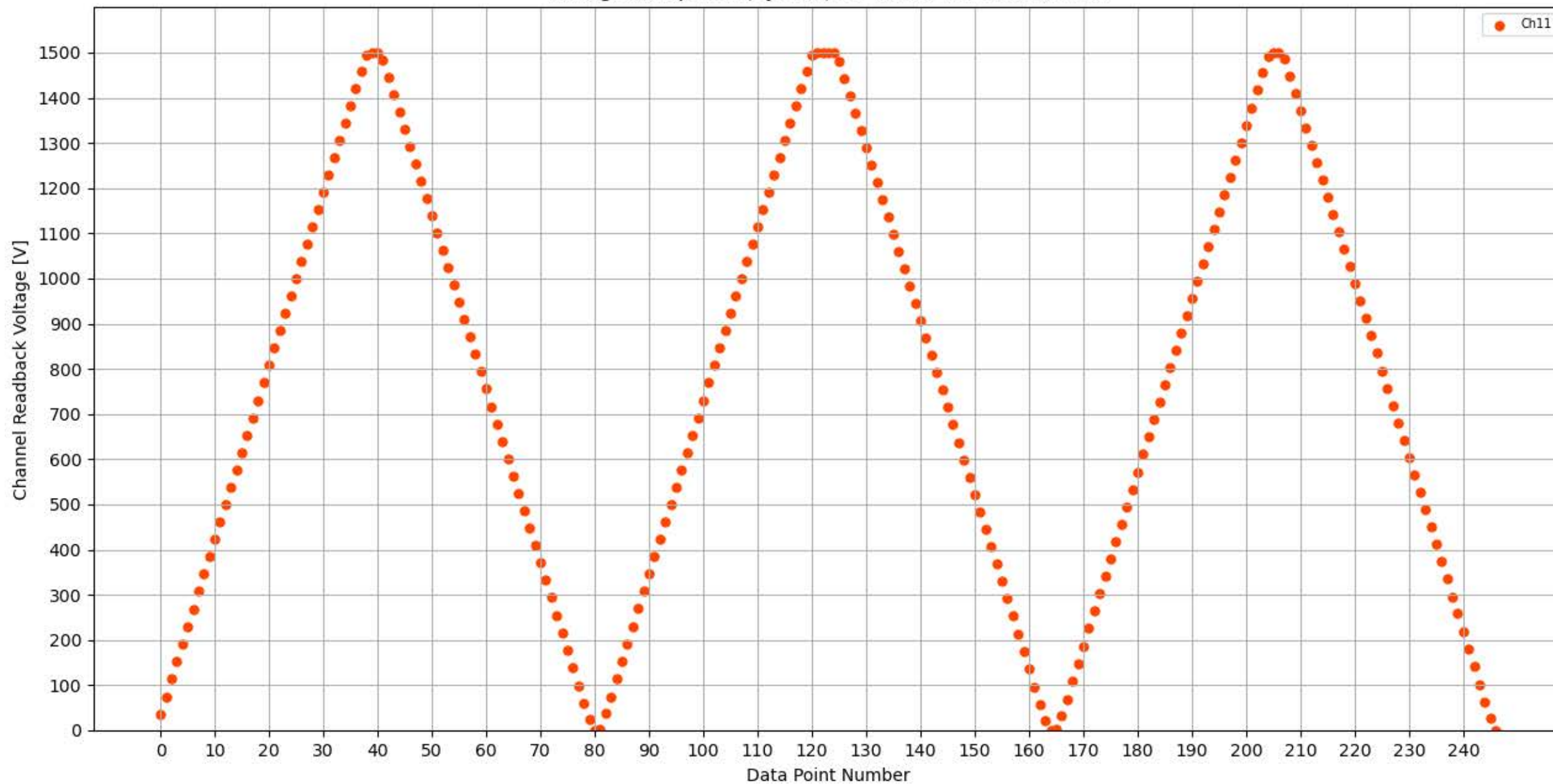
Voltage Ramp Test (Python) Bd #355, Slot #5, Ch #11
