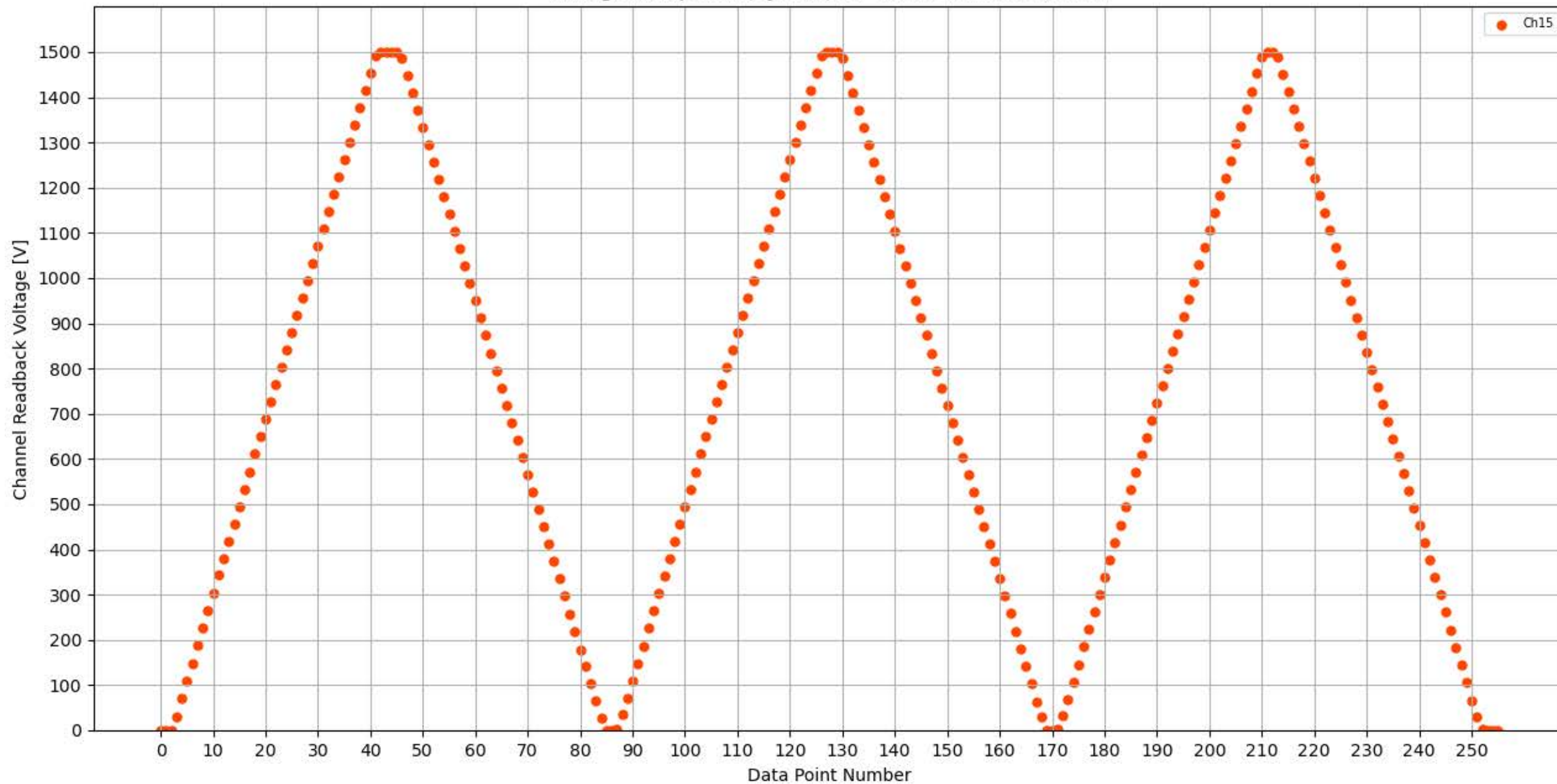
Voltage Ramp Test (Python) Bd #355, Slot #5, Ch #15
