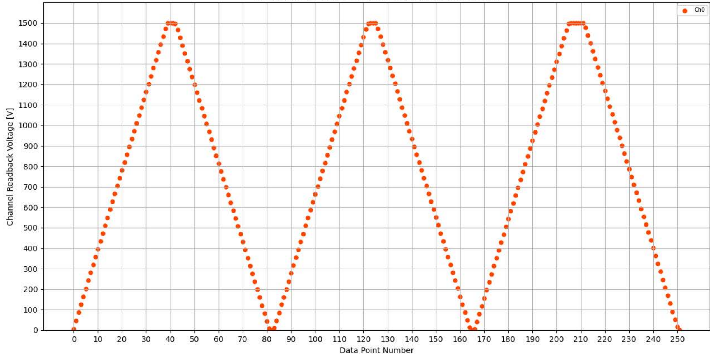
Voltage Ramp Test (Python) Bd #355, Slot #5, Ch #0
