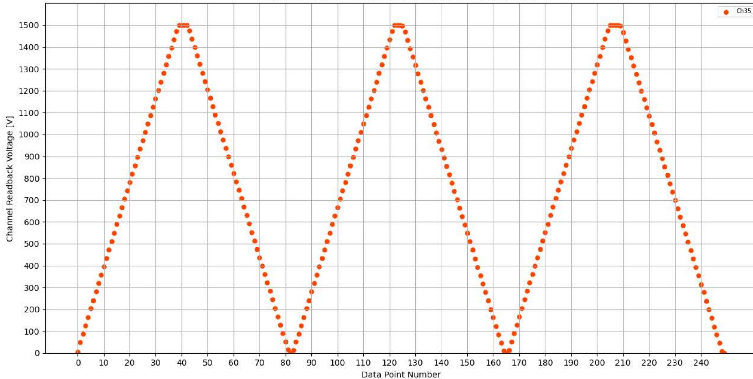
Voltage Ramp Test (Python) Bd #355, Slot #5, Ch #35
