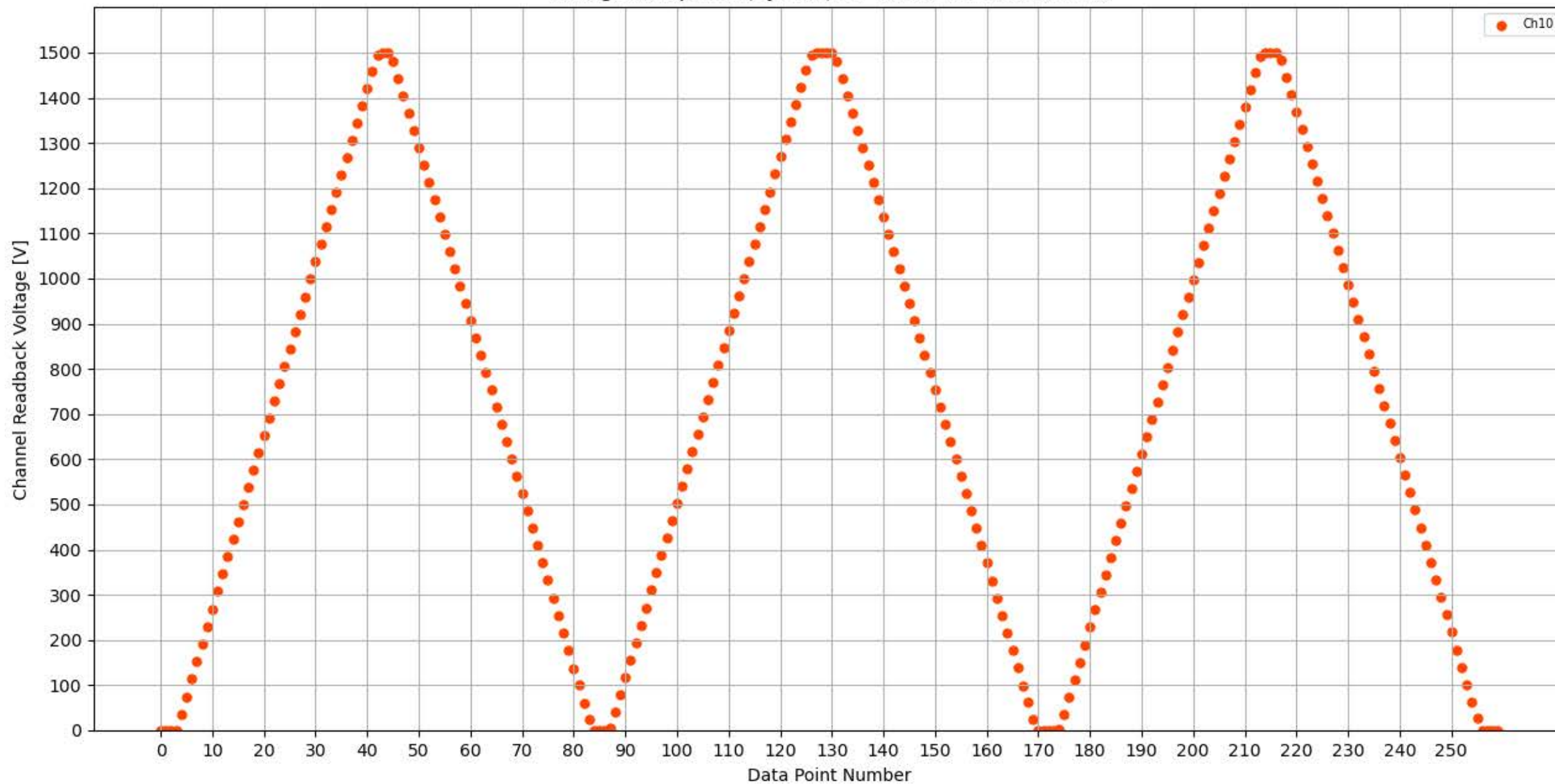
Voltage Ramp Test (Python) Bd #355, Slot #5, Ch #10
