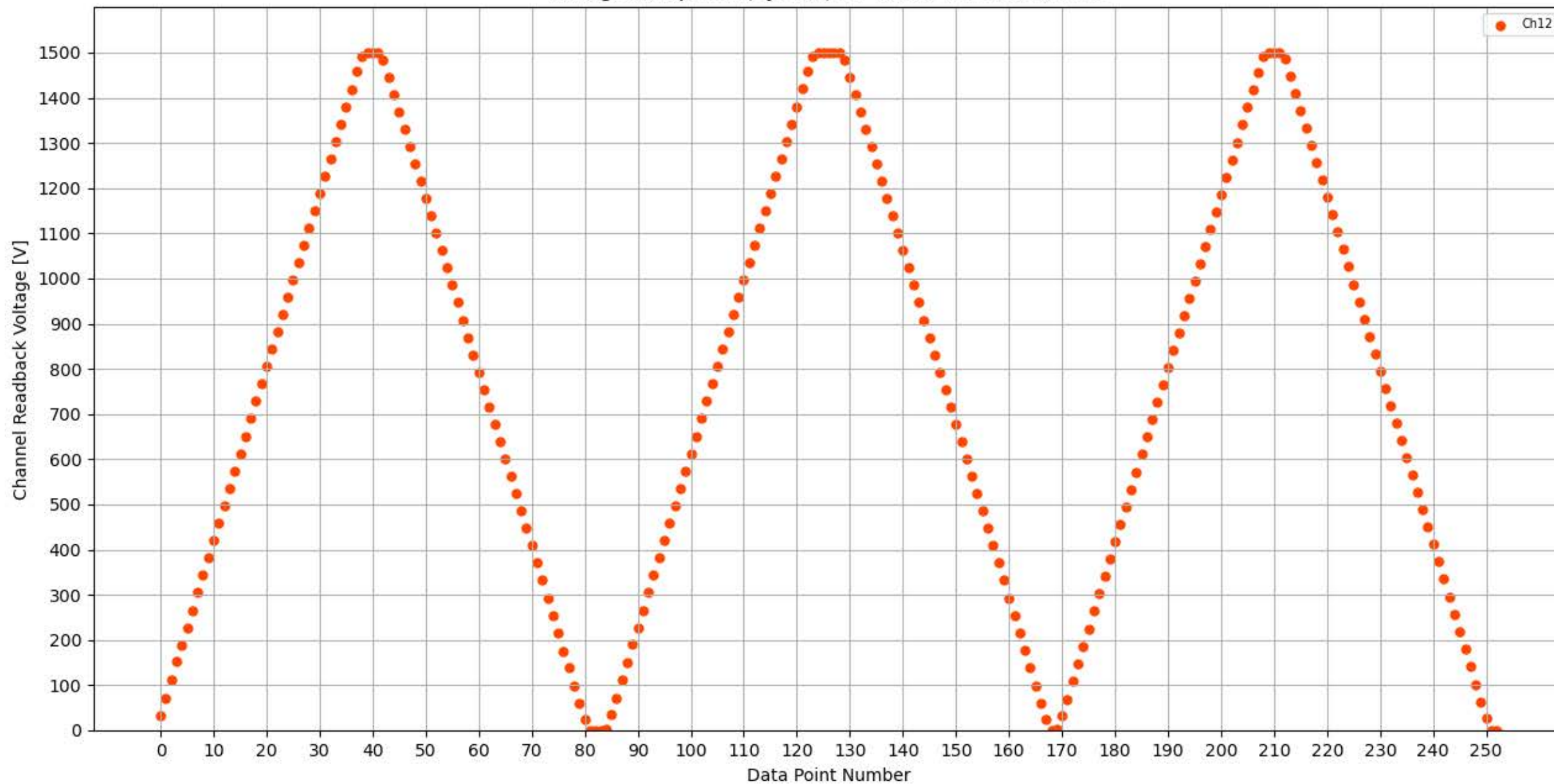
Voltage Ramp Test (Python) Bd #355, Slot #5, Ch #12
