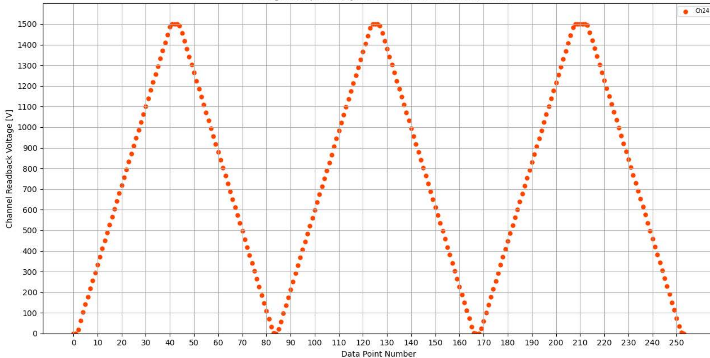
Voltage Ramp Test (Python) Bd #355, Slot #5, Ch #24
