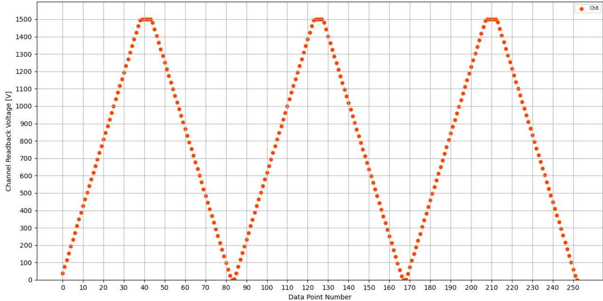
Voltage Ramp Test (Python) Bd #355, Slot #5, Ch #8
