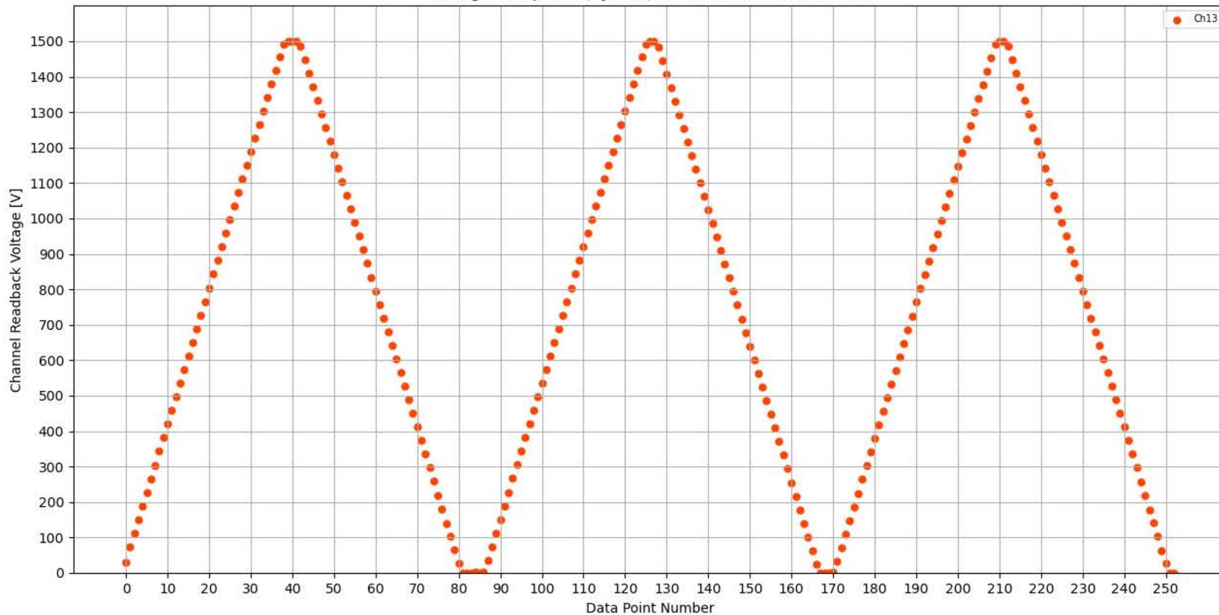
Voltage Ramp Test (Python) Bd #355, Slot #5, Ch #13
