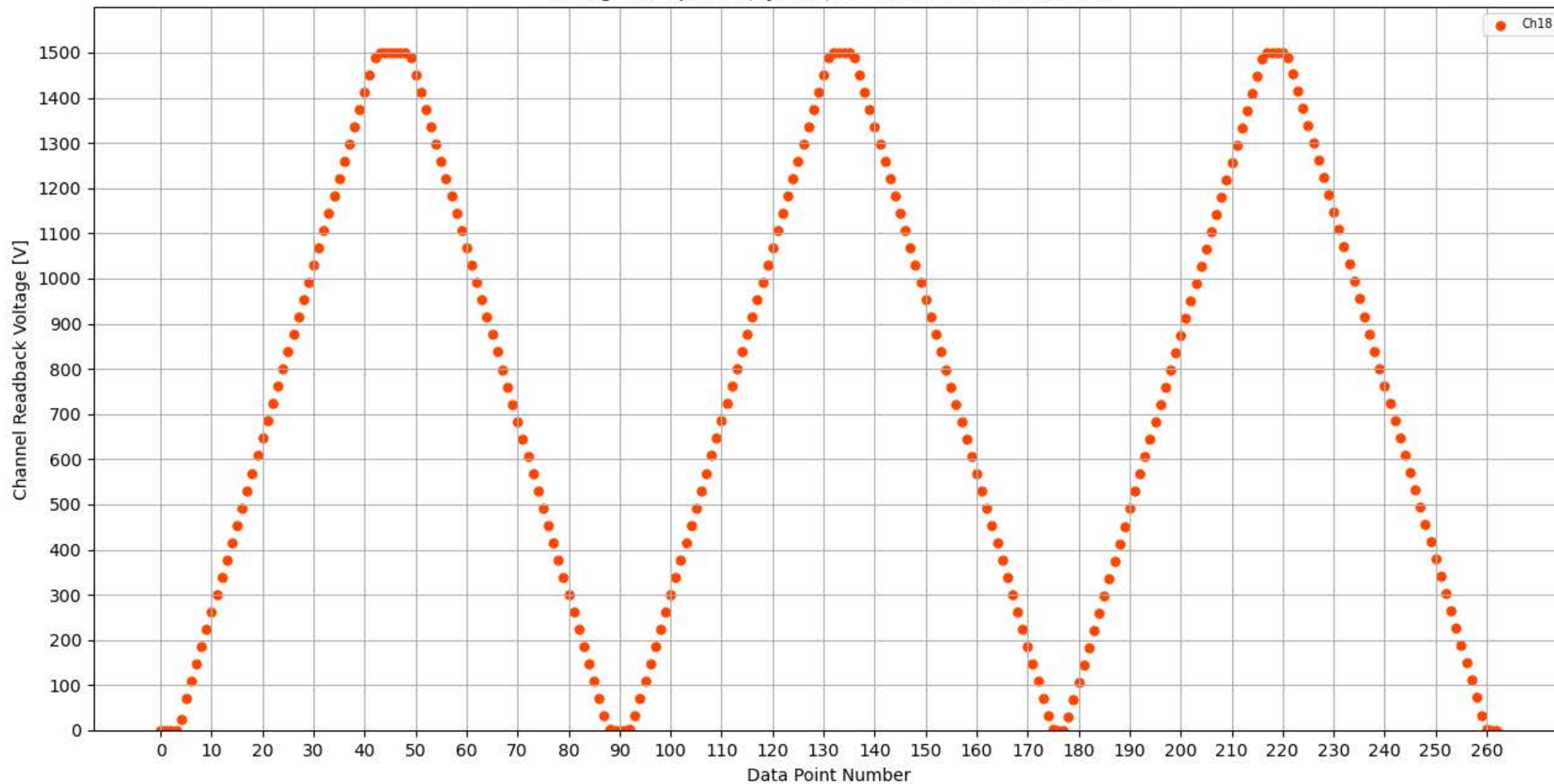
Voltage Ramp Test (Python) Bd #355, Slot #5, Ch #18
