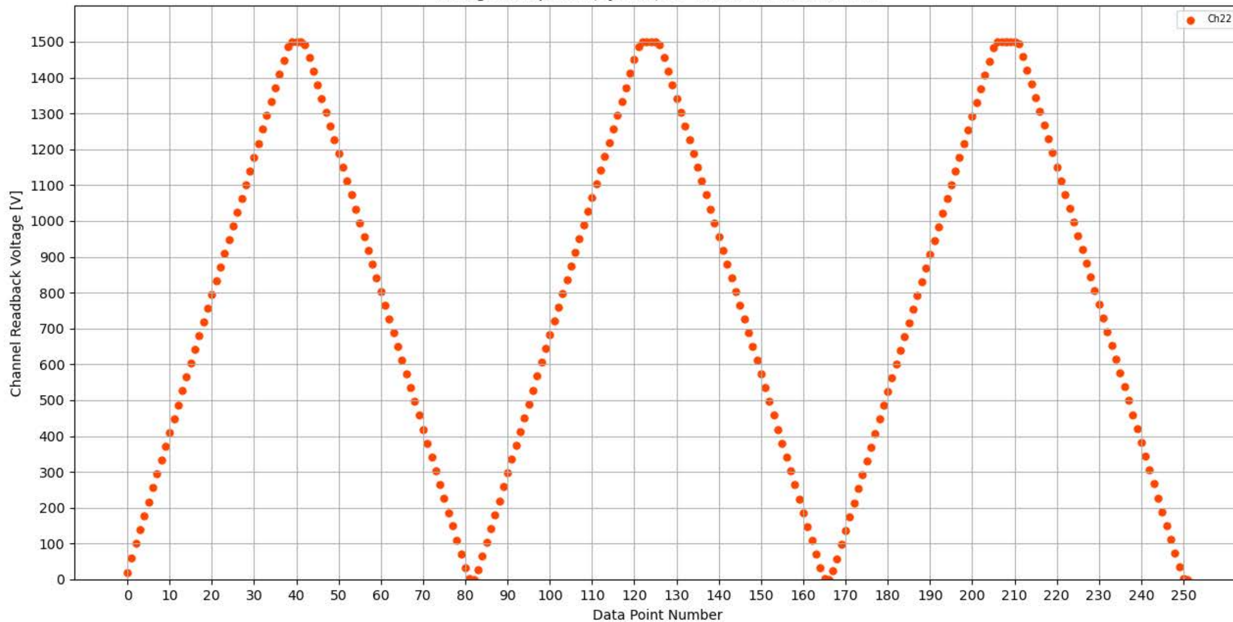
Voltage Ramp Test (Python) Bd #355, Slot #5, Ch #22
