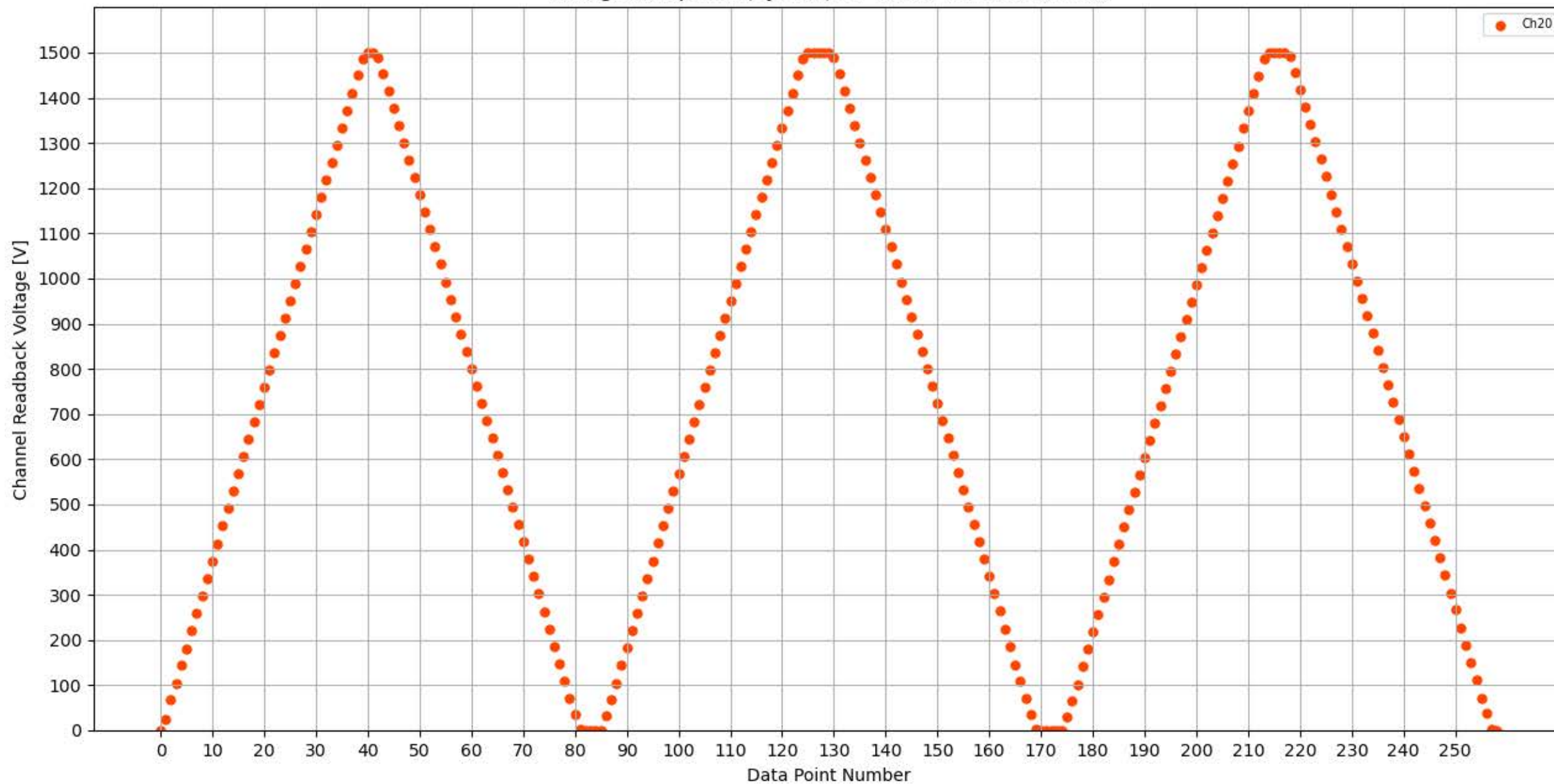
Voltage Ramp Test (Python) Bd #355, Slot #5, Ch #20
