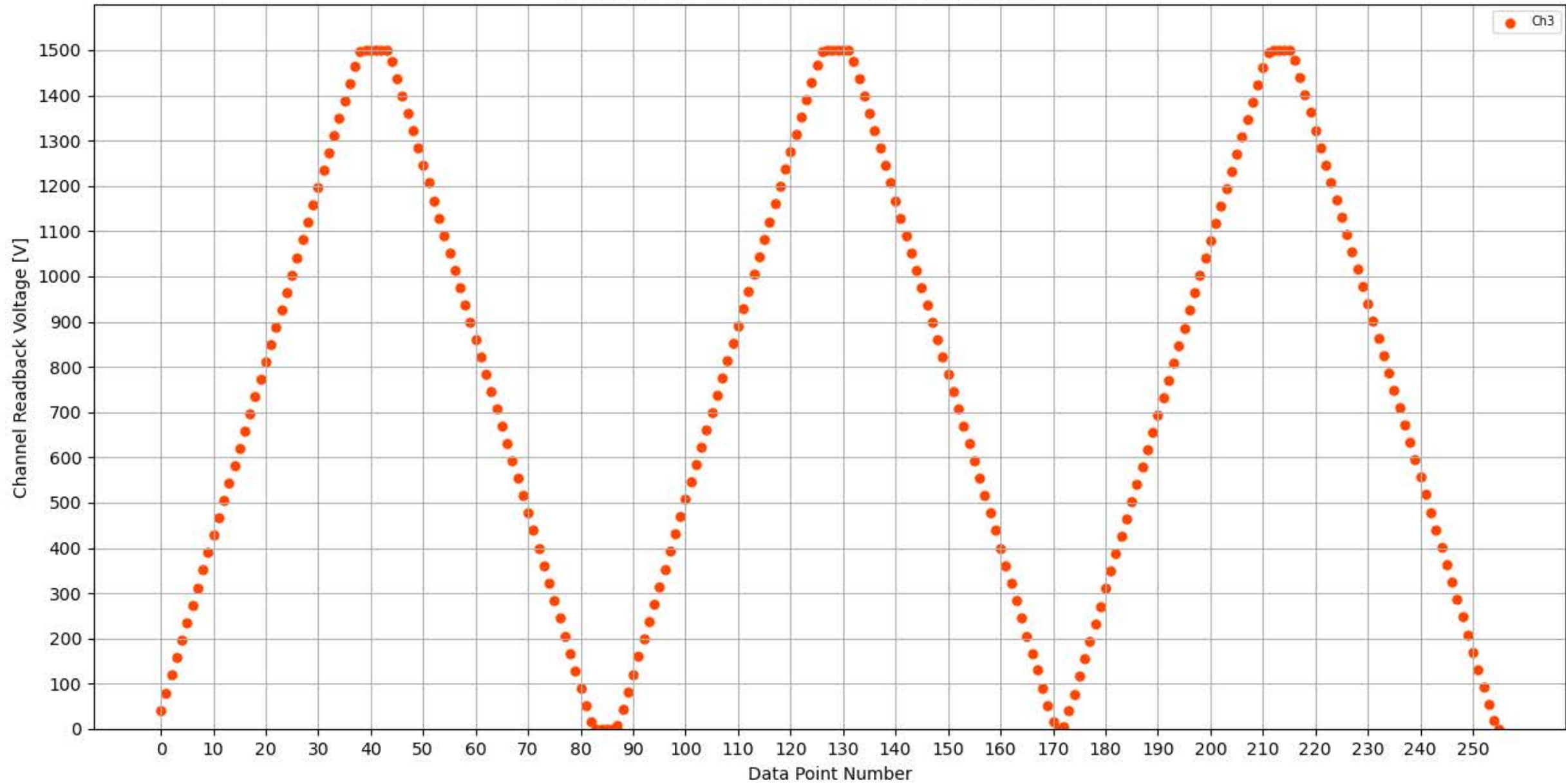
Voltage Ramp Test (Python) Bd #355, Slot #5, Ch #3
