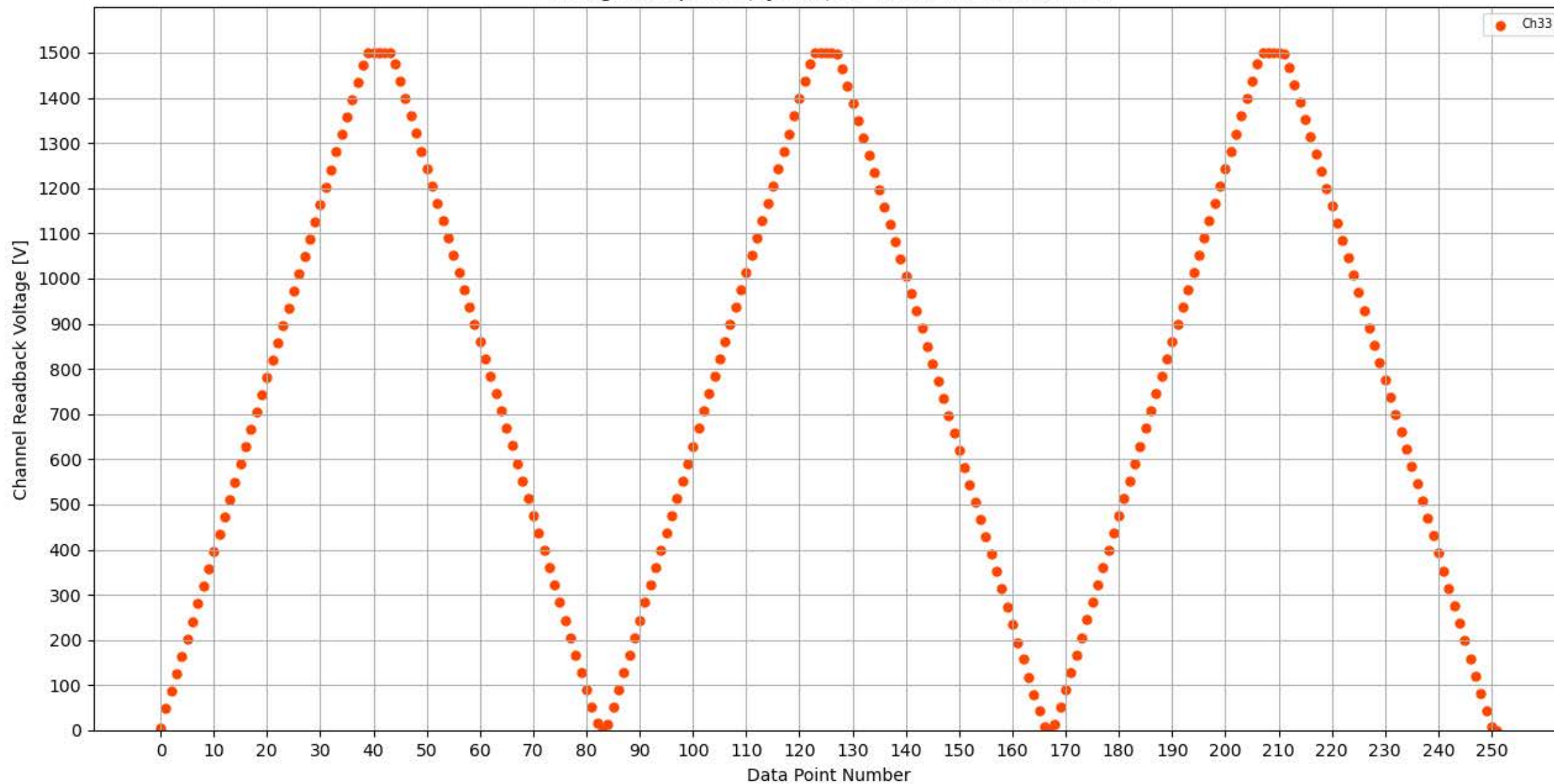
Voltage Ramp Test (Python) Bd #355, Slot #5, Ch #33
