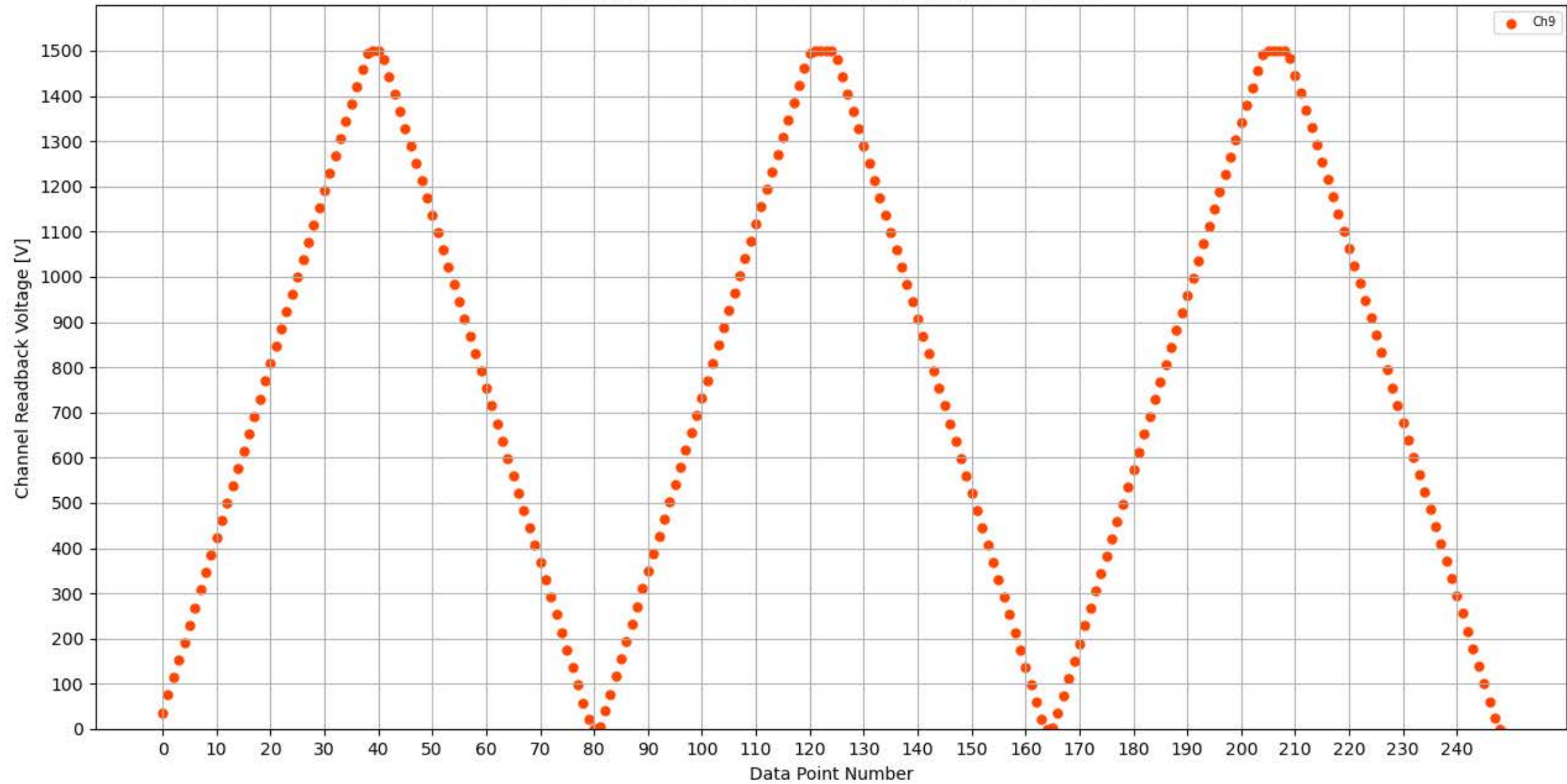
Voltage Ramp Test (Python) Bd #355, Slot #5, Ch #9
