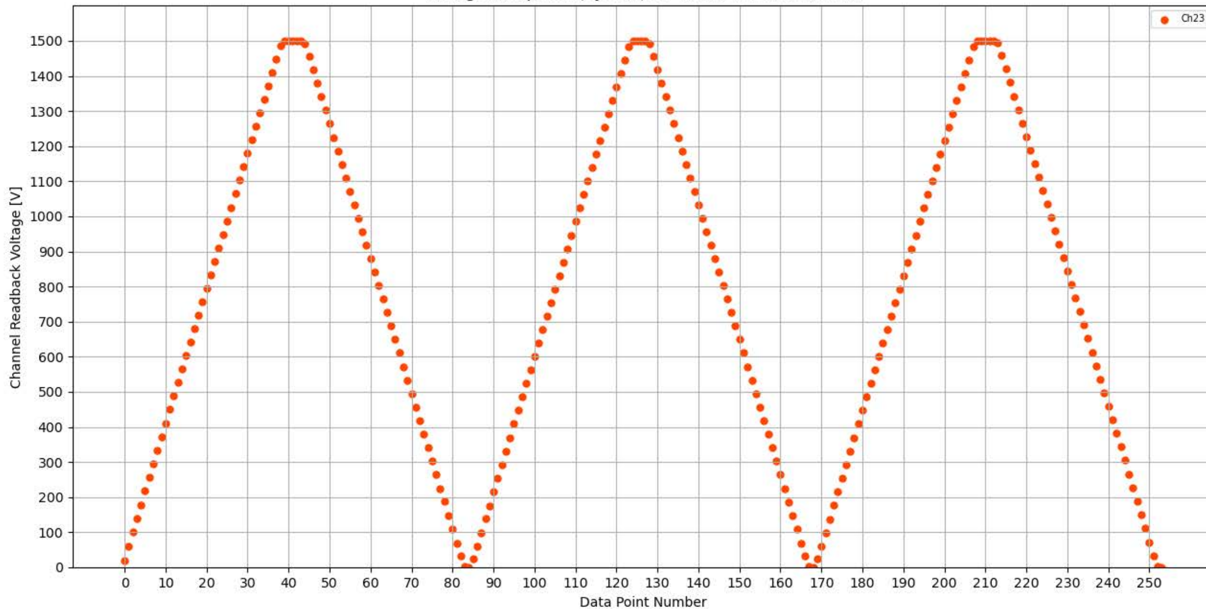
Voltage Ramp Test (Python) Bd #355, Slot #5, Ch #23
