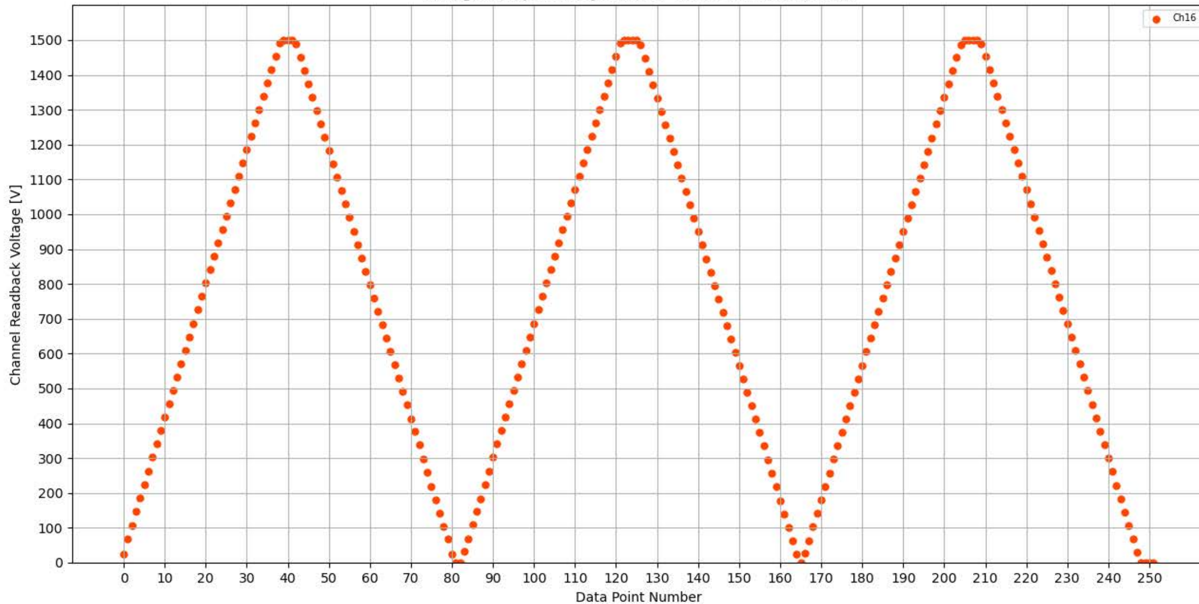
Voltage Ramp Test (Python) Bd #355, Slot #5, Ch #16
