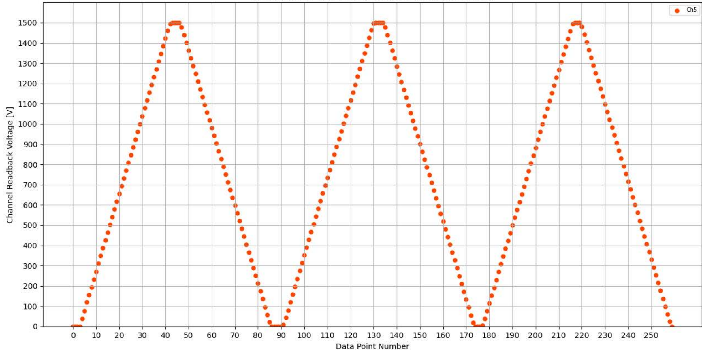
Voltage Ramp Test (Python) Bd #355, Slot #5, Ch #5
